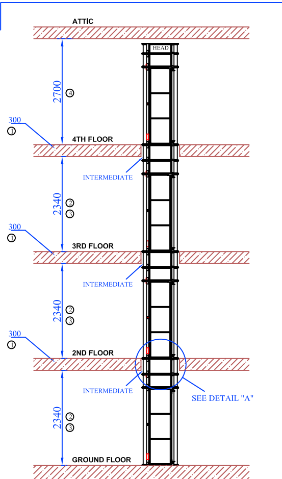
VIEW "A-A"
