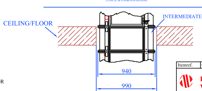
DETAIL "A" SCALE 2:1 (TYPICAL OF FLOOR PENETRATION)
