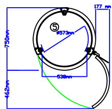
⑥ MAX. OPENING OF DOOR 90 DEGREE
