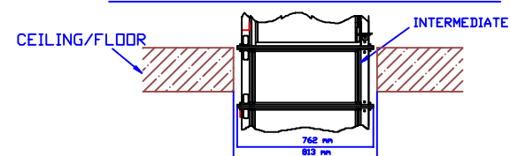
DETAIL "A" (TYPICAL OF FLOOR PENETRATION)
